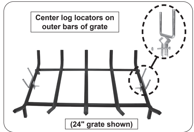
Fig. 17-1 Attach log locators to grate
