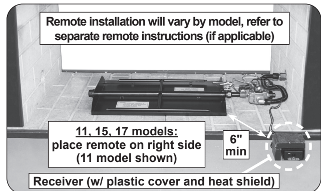
Fig. 16-2 Install remote receiver and/or heat shield (as applicable)
