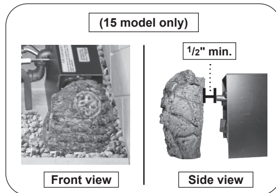
Fig. 20-2 Place wood chip (if applicable)
