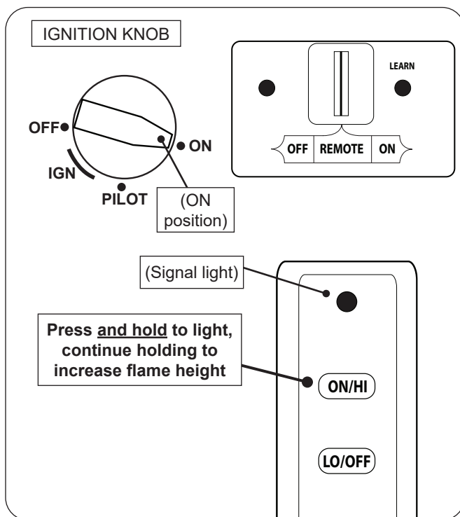
Fig. 32-1 Remote lighting
