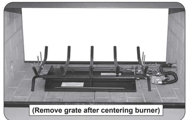
Fig. 17-2 Position grate
