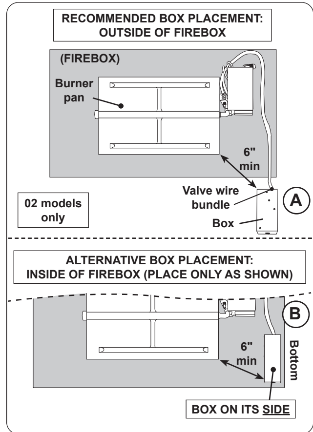
Fig. 16-1 Box placement (if applicable)
