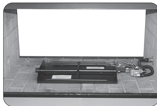
Fig. 15-2 Center burner in fireplace
