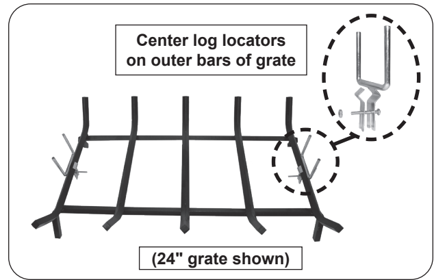
Fig. 11-1 Attach log locators to grate
