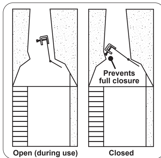
Fig. 8-2 Damper open / closed
