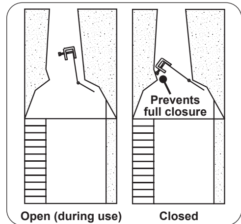
Fig. 10-2 Damper open / closed
