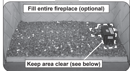
Fig. 20-1 Glass media placement
