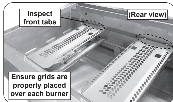
Fig. 31-1 Inspect heat distribution grids
