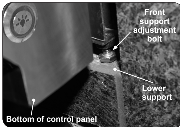
Fig. 28-2 Front support adjustment bolts
