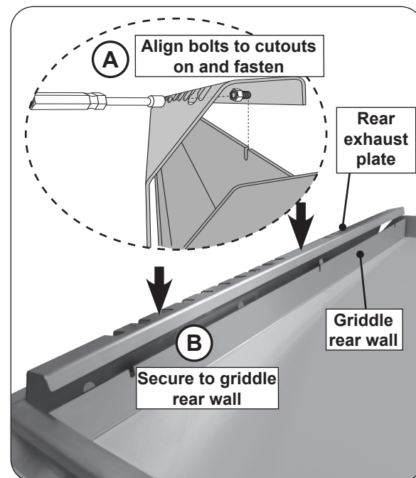
Fig. 31-4 Install rear exhaust plate
