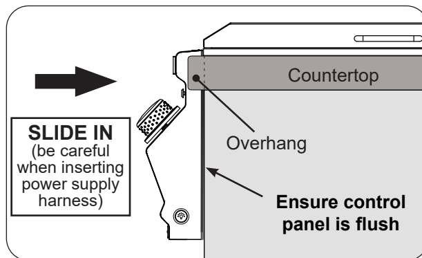
Fig. 28-1 Slide in unit (ensure flush)
