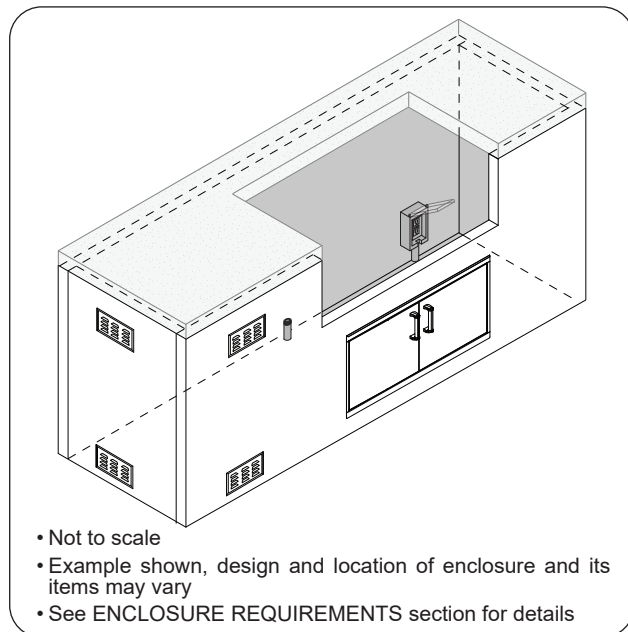
Fig. 27-1 Enclosure construction overview (if applicable)
