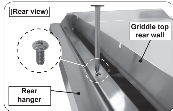
Fig. 31-3 Secure griddle top
