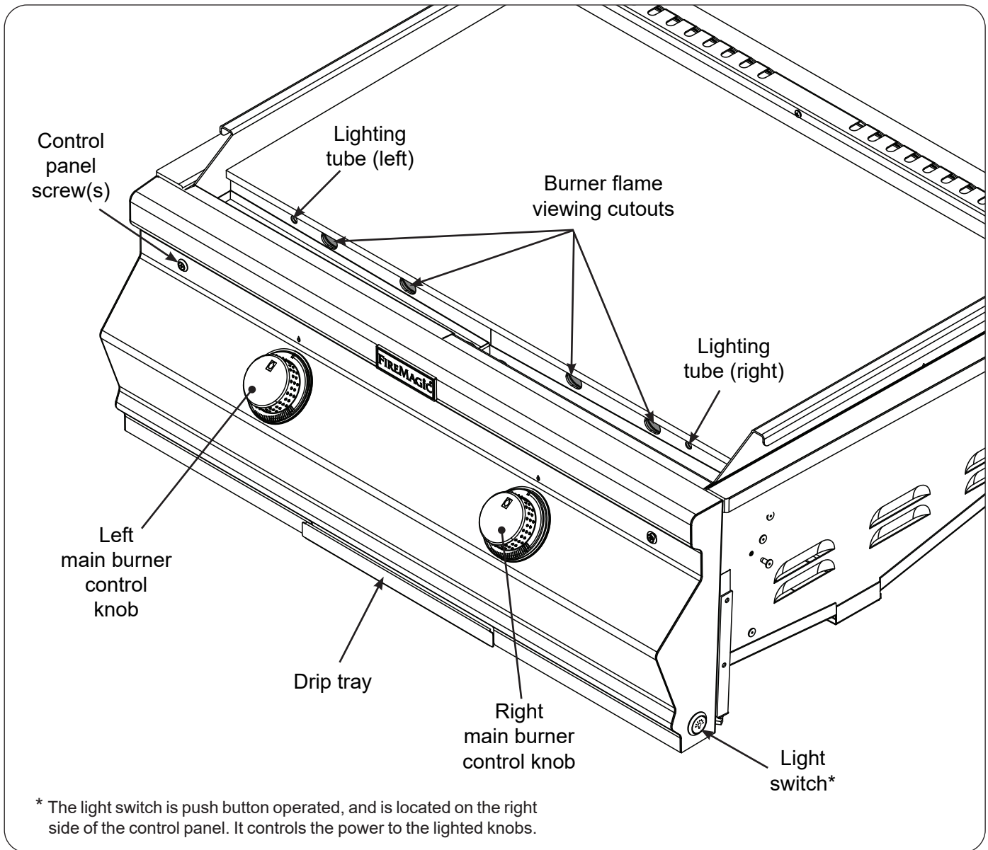
Fig. 33-1 A660i Griddle controls
