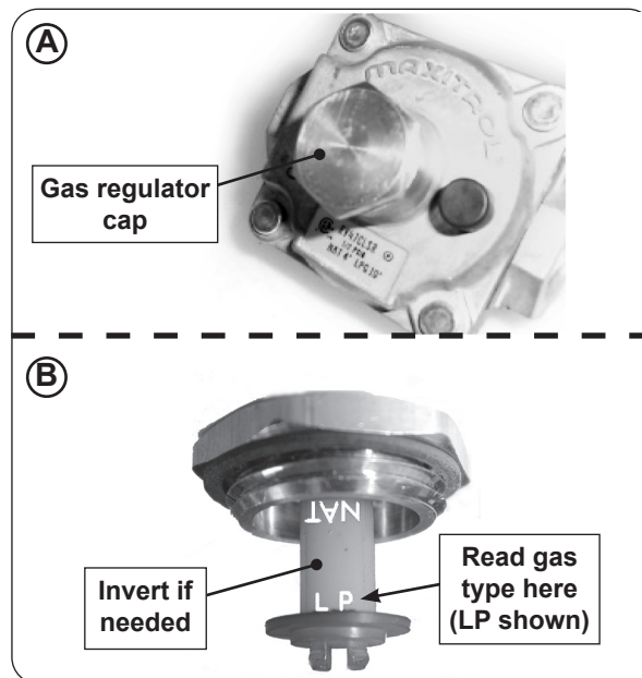
Fig. 42-1 Regulator conversion
