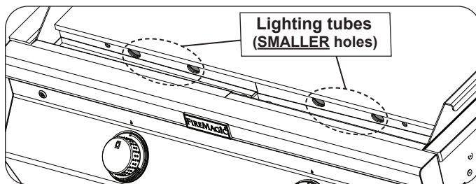
Fig. 35-2 - Burner flame viewing cutouts
