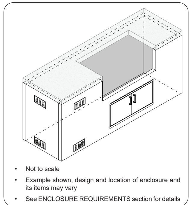
Fig. 23-1 Enclosure construction overview
