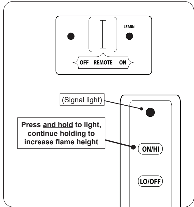
Fig. 35-1 Remote lighting
