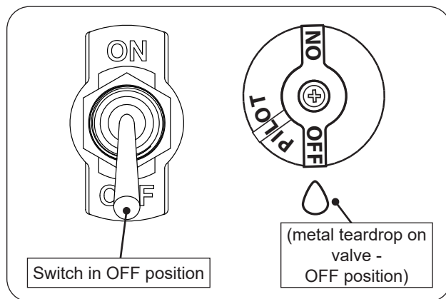
Fig. 28-2 Manual shut down
