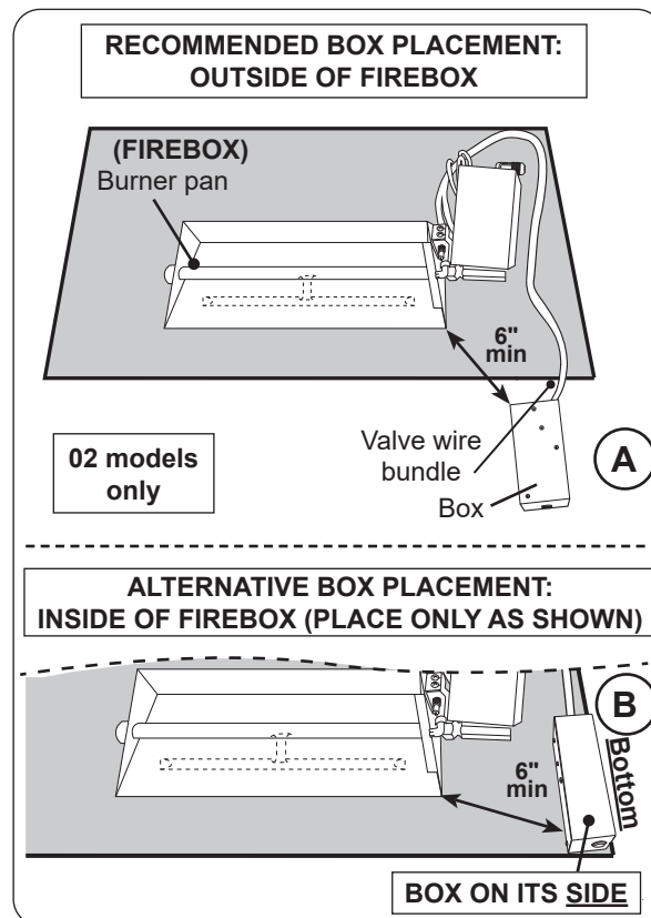
Fig. 17-1 Box placement (if applicable)
