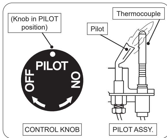
Fig. 23-1 Pilot lighting
