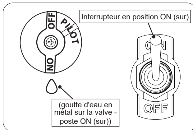
Fig. 48-1 Manual lighting
