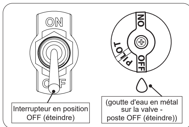
Fig. 48-2 Manual shut down
