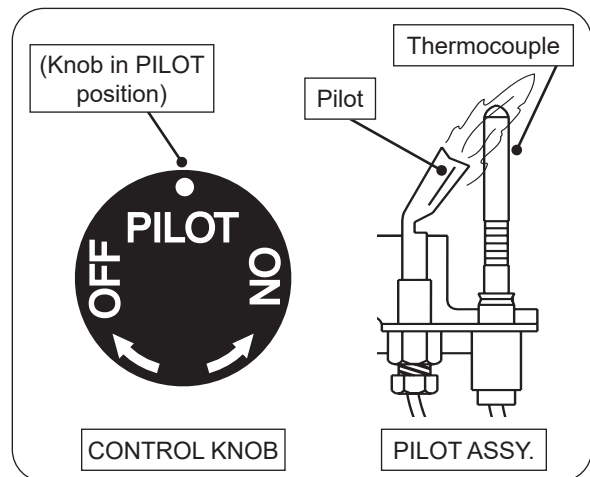
Fig. 33-1 Pilot lighting
